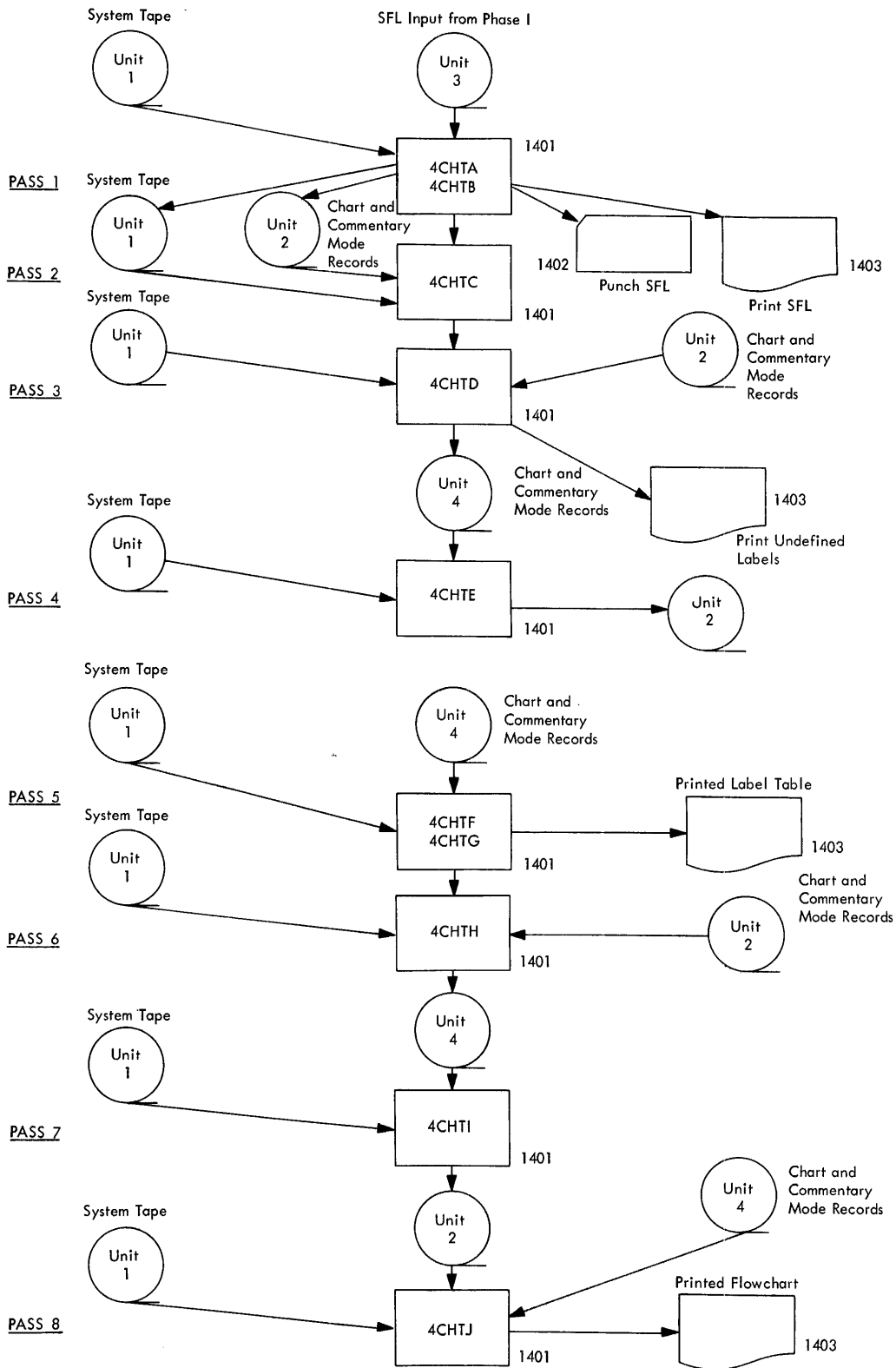
Flowcharter--Phase II
