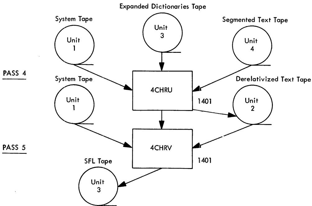
Flowcharter--Phase I
